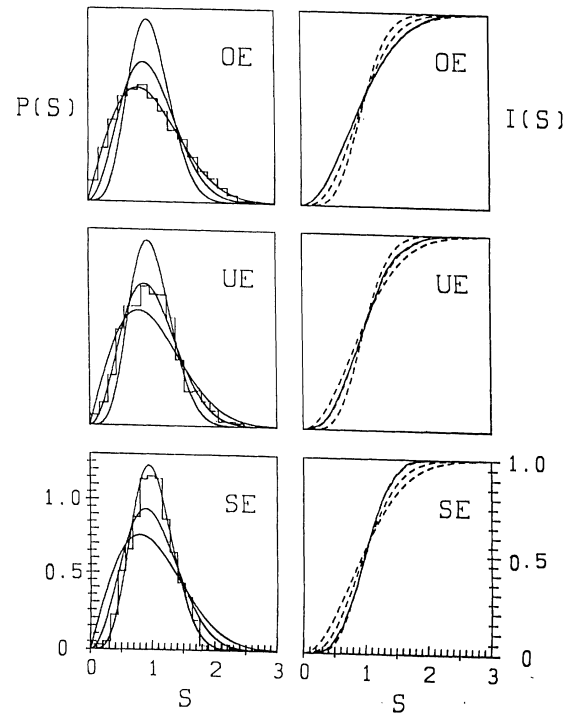
FIG. 1. The histogram on each of the plots in the left-hand column of the figure is the numerically computed distribution P(S) for the nearest-neighbor spacing S of the eigenvalues of the Hamiltonian corresponding to the ensemble marked on the plot. The solid curve with maximum height on each of the plots for the histograms is the P(S) for the Wigner surmise for the SE followed by that for the UE and OE. The solid curve on each of the plots in the right-hand column is the numerically computed staircase function I(S) as a function of S for the Hamiltonian corresponding to the ensemble marked on the plot. The dashed curves on each of those plots are the I(S) for the Wigner surmise. The dashed curve that is uppermost near S=0 in each of those plots is the Wigner surmise for the OE, followed by those for the UE and SE.
